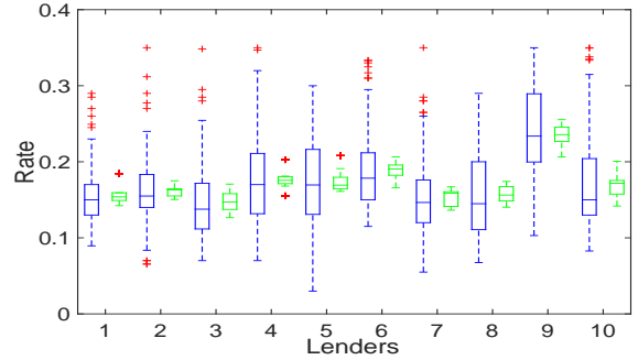
Figure 4: Rate v.s. single loan and portfolio.
