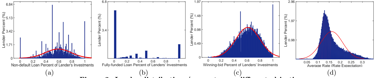
Figure 2: Lender distributions/percentages v.s. different objectives.
