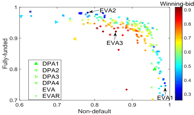
Figure 6: Solutions found by different algorithms. with more economic profits. SELF and several methods with low performances on non-default objective even get negative return rates on Return-0.6.
