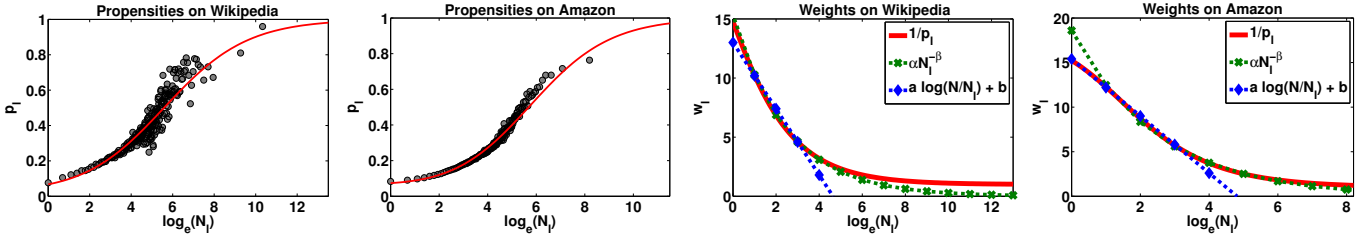
Figure 2: Propensities p_l and their corresponding weights w_l = 1/p_l on Wikipedia and Amazon. The estimated propensities follow a sigmoidal curve on the semi-log plot and provide a principled setting of the weights for recommending rare items as compared to popular heuristics such as N_l^{-\beta} and \log(N/N_l) .
