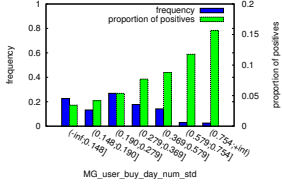
(c) merchant, rank 1
