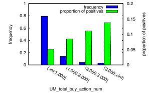
(b) user-merchant, rank 7
