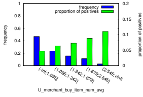
(a) user, rank 96
