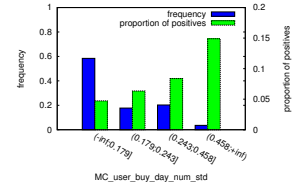
(f) merchant-category, rank 12
