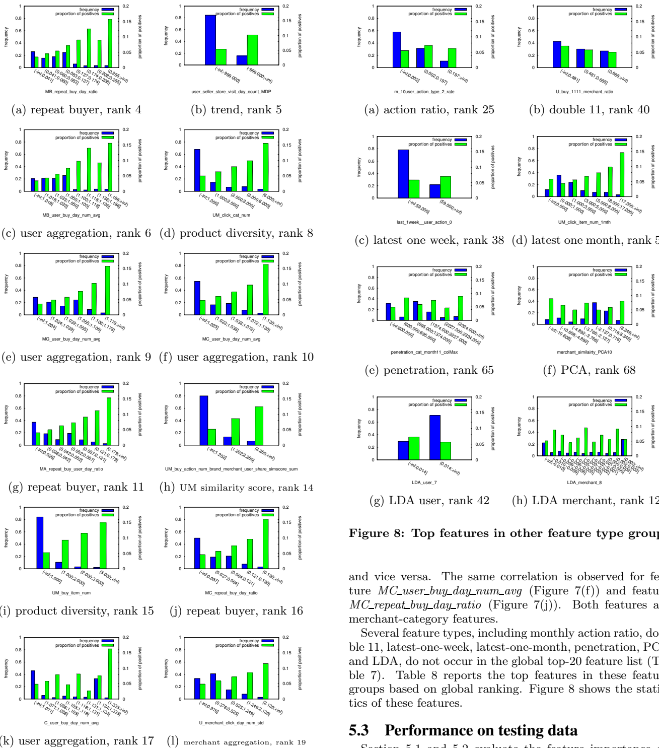
Figure 7: Features with high global ranking
