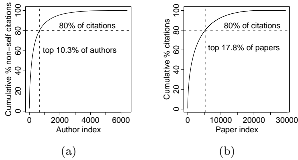
Figure 4: Cumulative percent of non-self citations received (a) per author and (b) per paper.
