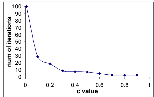
Figure 9: c value vs. number of iteration for converging for DBLP
