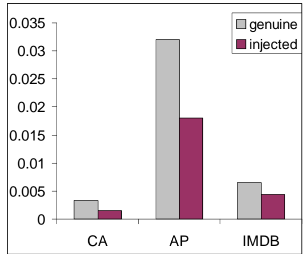
Figure 13: Normality scores between genuine and injected nodes across 3 datasets
