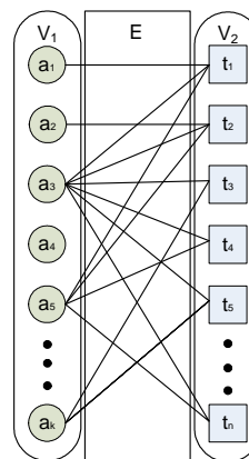
Figure 1: Bipartite Graph
