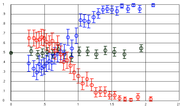
Figure 1: A graph of variable #1, which has a correlation of .006 with the target. The x axis represents the support of variable #1 and the y axis represents the probability of belonging to the positive target class.
