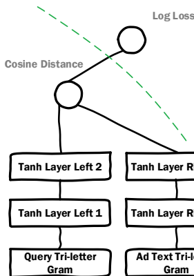
Figure 3: A DSSM Model with Log Loss
